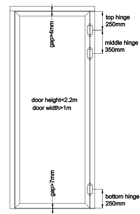
Over-width Door
