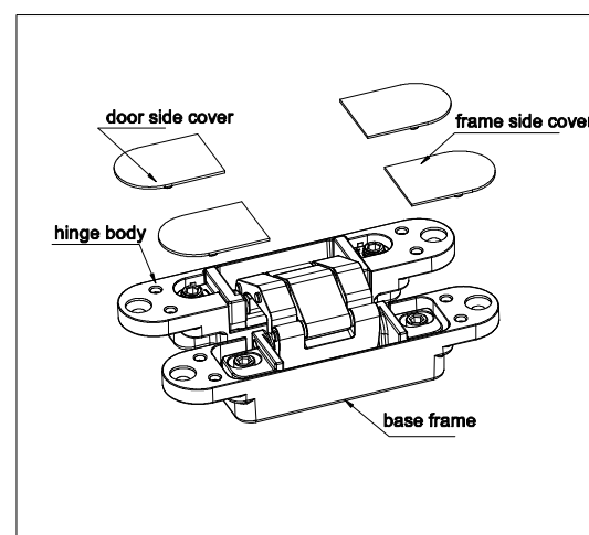
HINGE DETAIL
